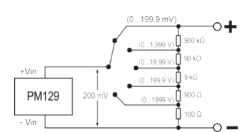
Connection diagram voltage decade
