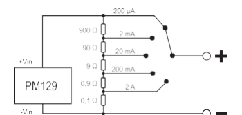
Connection diagram current decade
