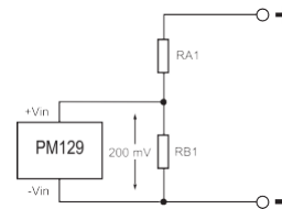
Principle Circuit
