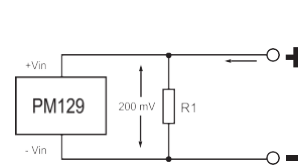
Principle Circuit
